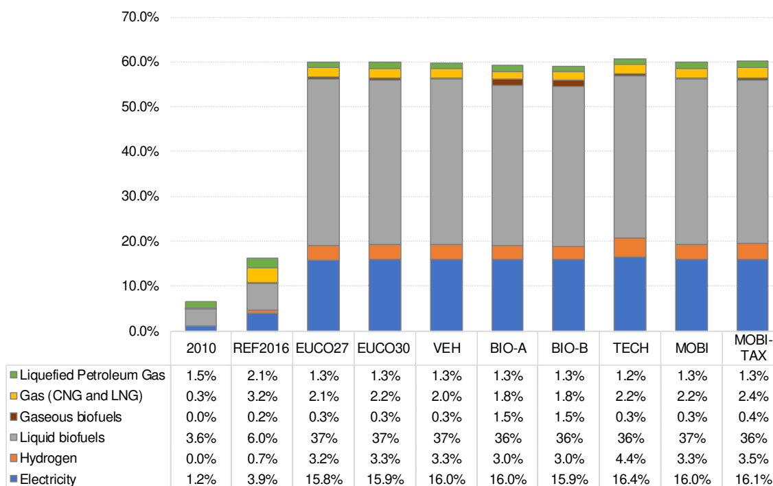
Figure 52: Alternative fuels/energy sources in transport in 2050 (in % of total energy demand)
