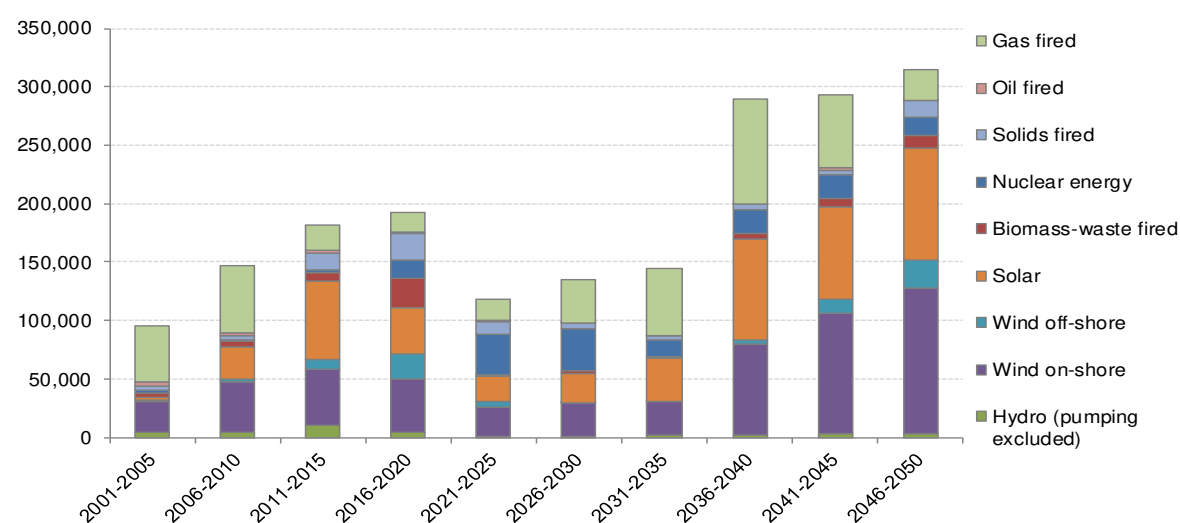
Figure 35: Net power capacity investments by plant type (MWh – for five year period)
