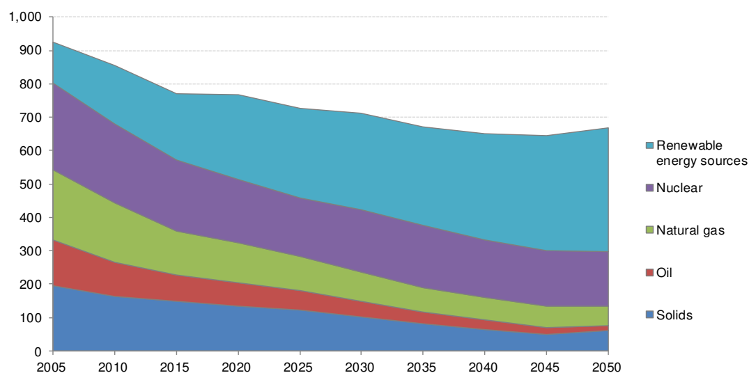
Figure 32: EU28 energy production (Mtoe)
