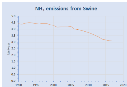
Figure 5-3 Calculated emissions for NH 3 from 1990 till 2018 for Swine in Greece.
