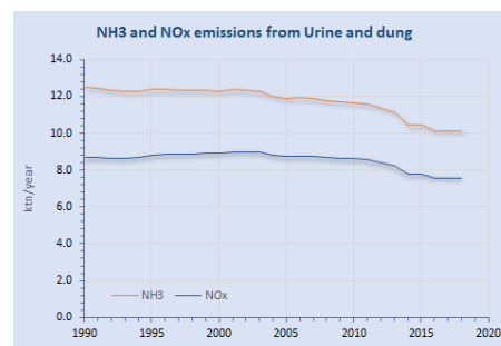
Figure 5-6 Calculated emissions for \text{NH}_3 and \text{NO}_x from 1990 till 2018 from Urine and dung deposited by grazing livestock in Greece.
